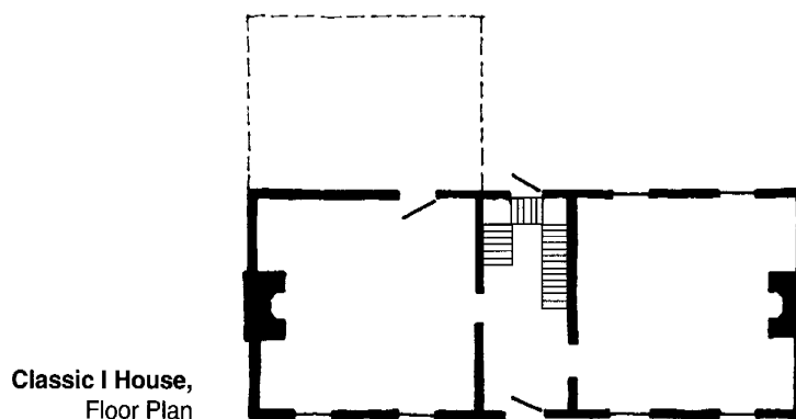
Classic I House , Hannan House, Gallia County, ca. 1840
