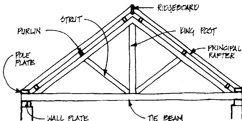
Roof Structure
